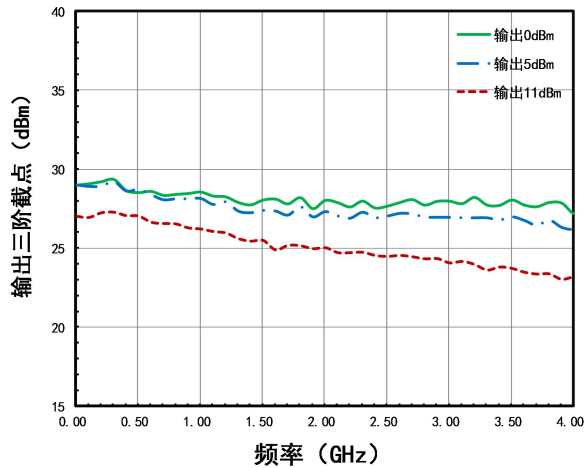
典型测试曲线: (50Ω系统, V_{dd}=+5V , I_{dd}=69mA )
